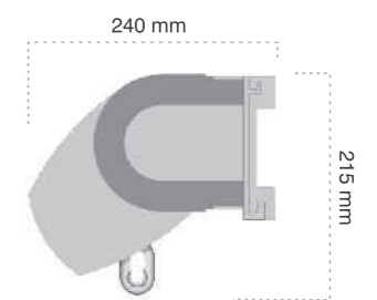
profilo terminale terminal profile
